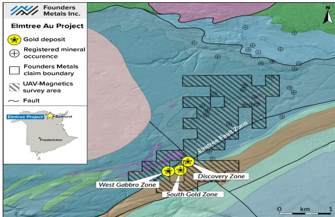
Figure 2: Map showing UAV magnetism survey coverage (hatched area). The regional geology overlay shows the coincidental nature of known gold mineralization with the Elmtree Fault Zone.
