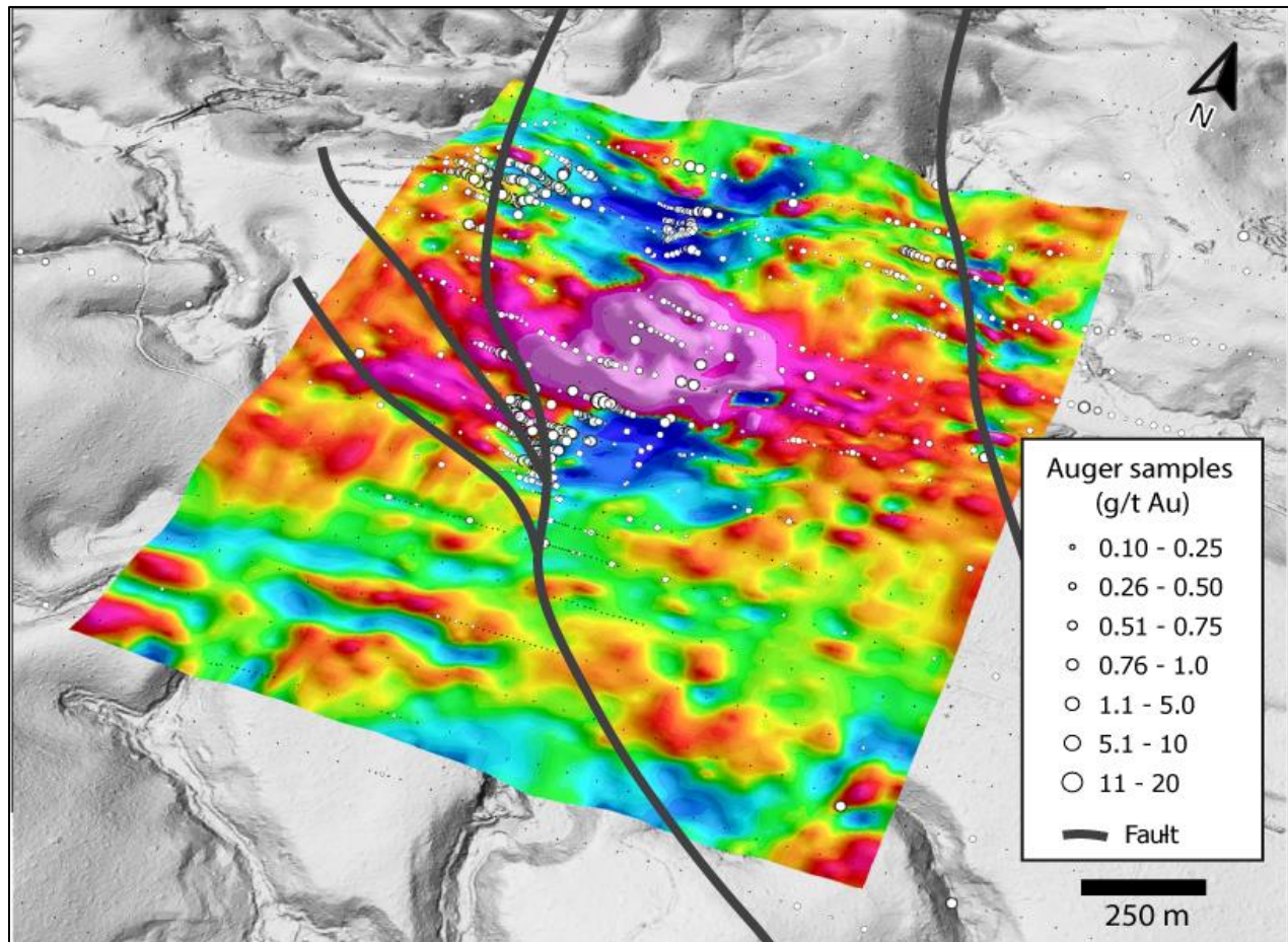
Figure 6: Ground Magnetics Survey of Upper Antino
